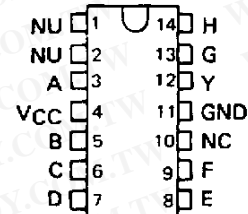
SN54LS54 . . . J OR W PACKAGE SN74LS54 . . . D OR N PACKAGE (TOP VIEW)
