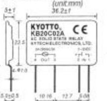
OUTLINE DIMENSIONS (unit:mm)
