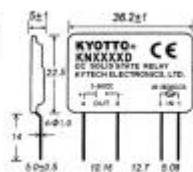
OUTLINE DIMENSIONS (mm:INCH)
