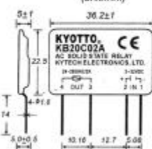
OUTLINE DIMENSIONS (unit:mm)
