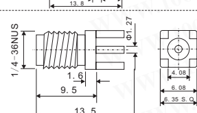
SMA jack PCB mount
