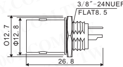
BNC female isolated ground bulkhead
