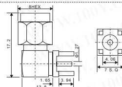
SMA plug PCB mount right angle
