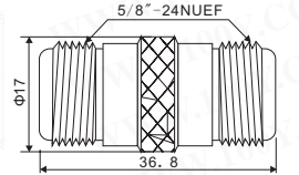
N female to N female
