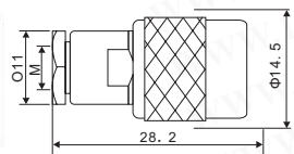
TNC male clamp type
