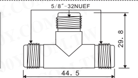
N three female
