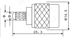
TNC male crimp
