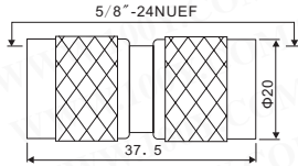
MC 1-7321 N male to male (UG-57B/U)
