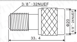
N male to F female
