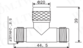
N male to double N female
