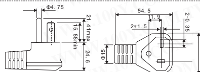
3P Computer Power Cord
