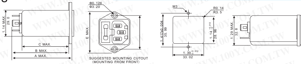
SUGGESTED MOUNTING CUTOUT (MOUNTING FROM FRONT)
