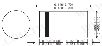
MINI-MELF SOD-80/DO-213AA
