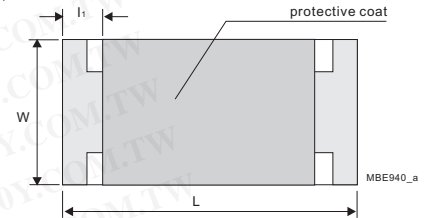
Fig. 3 Chip resistor construction
