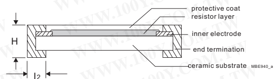
Fig. 4 Chip resistor construction
