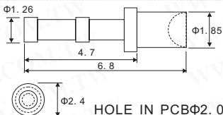
HOLE IN PCB \Phi 2.0
