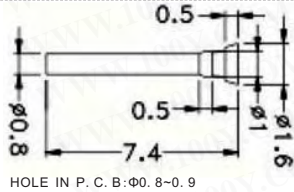
HOLE IN P. C. B: \Phi 0.8-0.9
