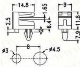
MOUNTING HOLES
