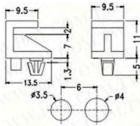
MOUNTING HOLES
