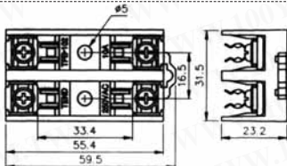
Rail- Fuse Holder
