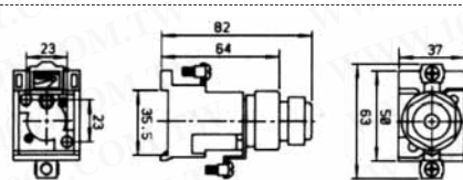
Rail- Fuse Holder
