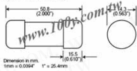
Fig. 1: 1-50 Amp Range
