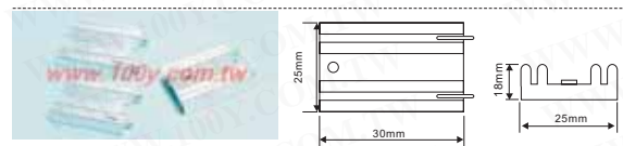
Dual In Line Heat Sink
