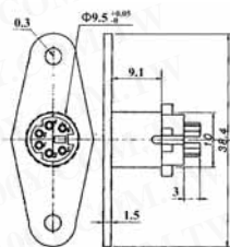
Unit: mm
