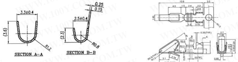
Unit: mm
