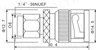
SMA male to BNC male
