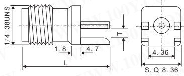
SMA jack PCB mount
