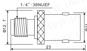
SMA female to BNC female
