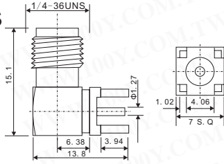
SMA plug PCB mount right angle
