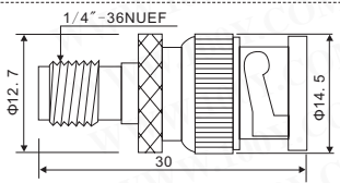
SMA female to BNC male
