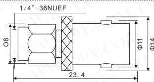
SMA male to BNC female
