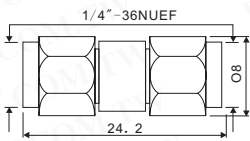
SMA double male
