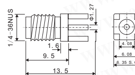
SMA jack PCB mount
