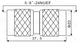
MC 1-7321 N male to male (UG-57B/U)
