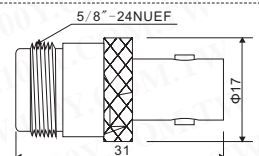
MCI-7068 BNC FEMALE TO N FEMALE
