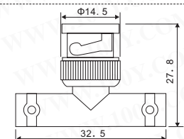
MCI-7077 BNC MALE TO DOUBLE BNC FEMALE
