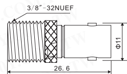
MCI-7066 BNC FEMALE TO F FEMALE
