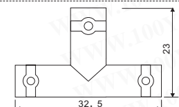
MCI-7080 BNC THREE FEMALE
