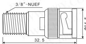
MCI-7050 BNC MALE TO F FEMALE
