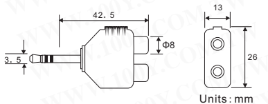
A: 3.5mm stereo plug to 2x3.5mm mono jacks B: 3.5mm stereo plug to 2x3.5mm stereo jacks
