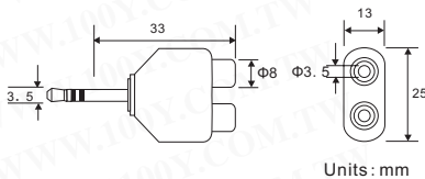
3.5mm 1/4 stereo plug to double RCA jack
